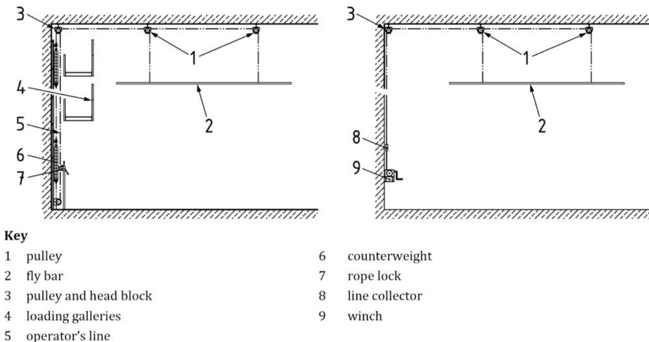
Figure 7 — Examples of manual systems
