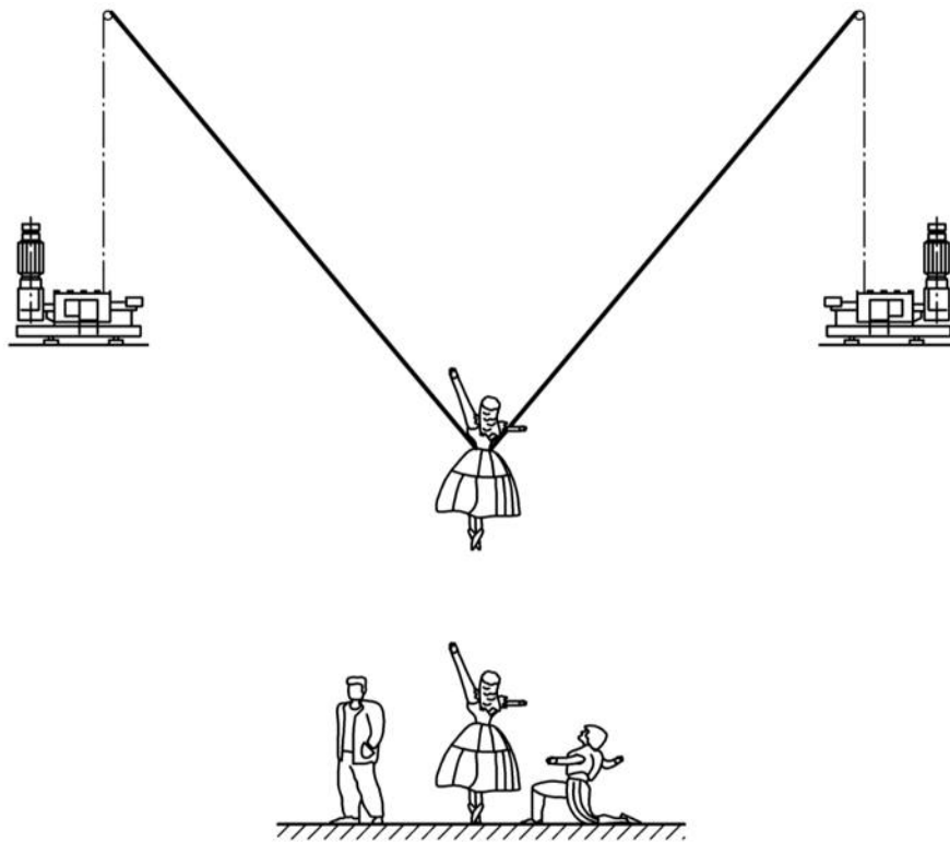
Figure G.5 — Two winches to fly a performer
